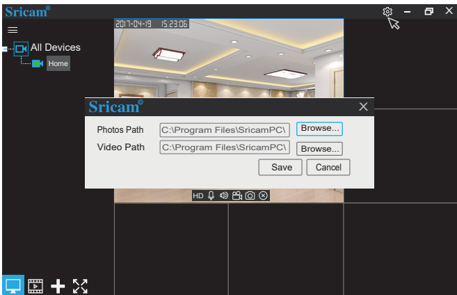
Figure 8 Path tab
