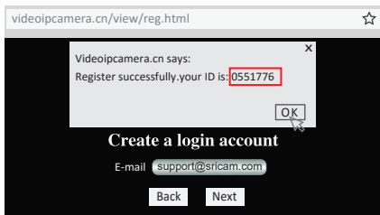
Figure 16 Account ID
