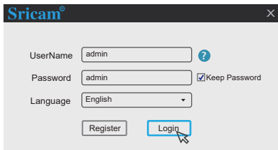
Figure 1 Login Window
