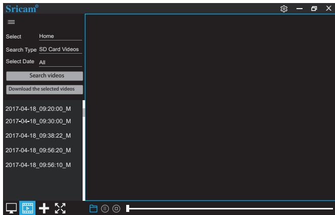
Figure 10 Playback
