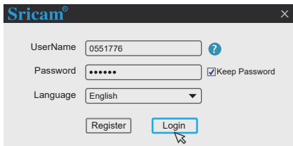
Figure 17 Login Window
